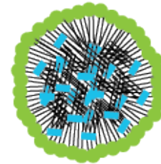
Figure 44: Schematic of a lipid droplet. Amphipathic phospholipids are shown in green, while neutral lipids such as cholesterol esters and triglycerides are shown in blue. The outside of the droplet allows it to be soluble in water, while the inside is hydrophobic.
